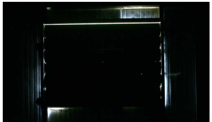
Figure 24. Whilst this store looks well constructed, major air-leakage points can be seen inside the store when dark
